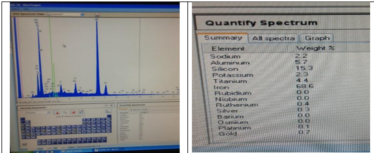
Different position in the iron rich mineral with 0.5 % PGM's and 0.7% Au
