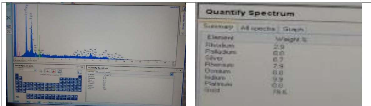
SEM result for gold button produced from pulps, 78.6% Au and 20.7% PGM's.
