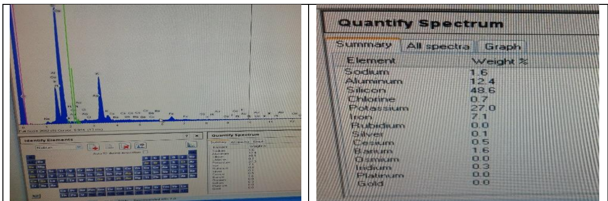
Shot on the edge of the mineral, showing 0.3% PGM's
