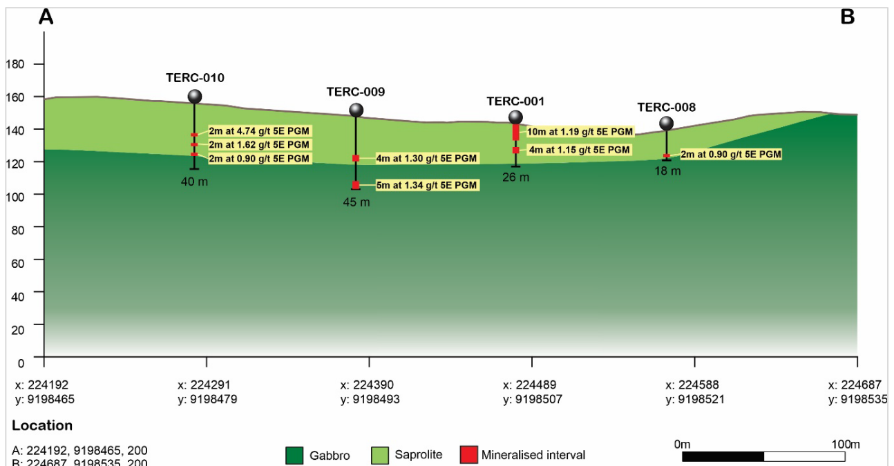
Figure 1 – A-B cross section with TERC-009 and TERC-010, down hole length reported, true width not known.
